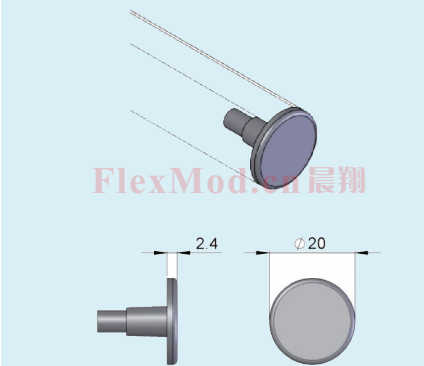
CXGEC 20 Distance Tube End Cap Polyamide (20mm 铝管端盖, 尼龙)
