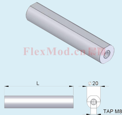
CXGRT 20x100 Distance Tube, L = 100mm Aluminium(支架横管长度100mm, 铝)
