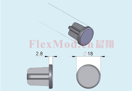
CXGEC 18 18mm Tube End Cap Polyamide (18mm 铝管端盖, 尼龙)
