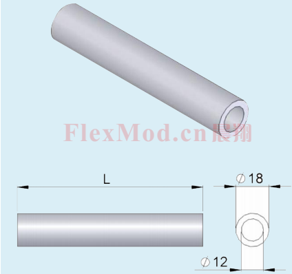
CXGRT 18x100 18mm Tube, L = 100mm Aluminium (支架竖管长度100mm, 铝)
