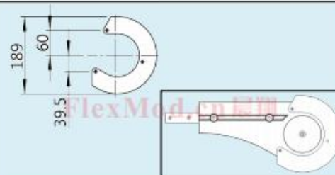
CXMSJ 189 Protective cover for idler end nit (尾端防护罩)
