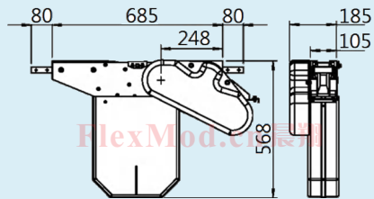
CXHEC 0HL Drive unit (驱动单元) Transmission on left-hand side (传动装置在左侧)
