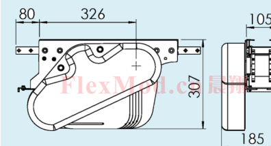
CXHER 0HR Drive unit (驱动单元) Transmission on right-hand side (传动装置在右侧)
