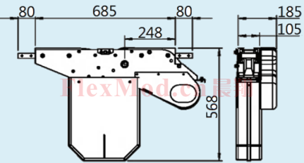
CXHEC 0HR Drive unit (驱动单元) Transmission on right-hand side (传动装置在右侧)
