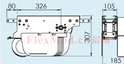
CXHER 0HL Drive unit (驱动单元) Transmission on left-hand side (传动装置在左侧)
