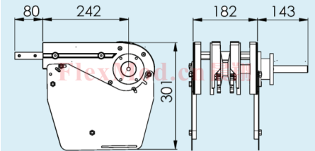
CXBEB 0A175LU Drive unit (驱动单元) Transmission on left-hand side (传动装置在左侧) SEW SA37 SEW WA 30 SEW WA 20
